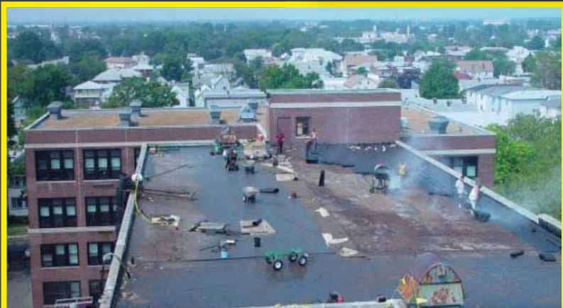
Roof Replacement
